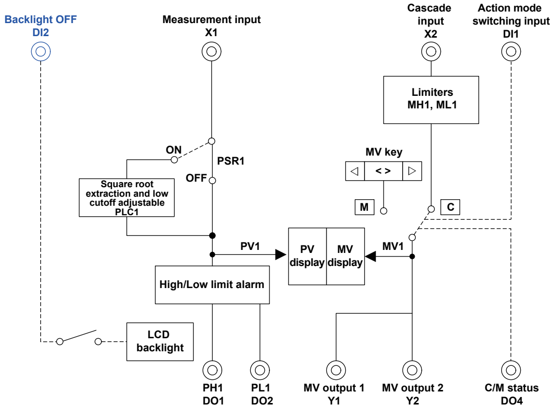
YS1360 functional block diagram
