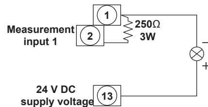
Connection of Transmitter Power Supply
