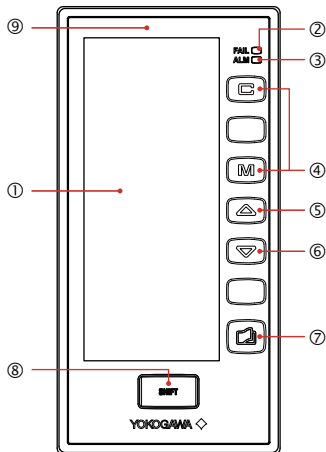
YS1350 front panel
