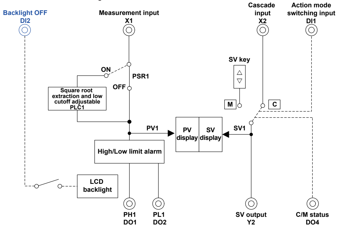
YS1350 functional block diagram
